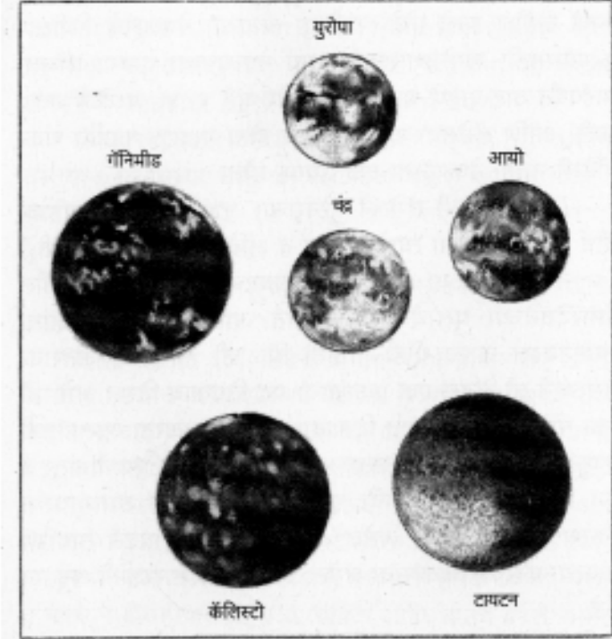
The Six Largest Satellites
